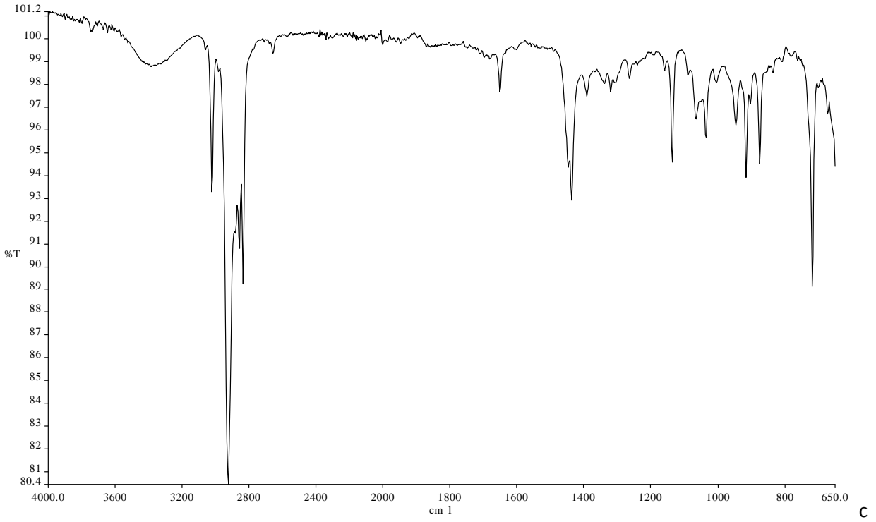
cyclohexene standard
