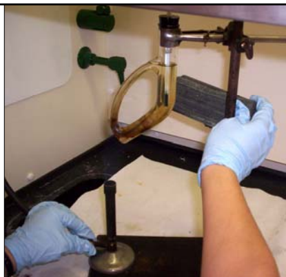
Melting Point Determination - the Thiele Tube Method
